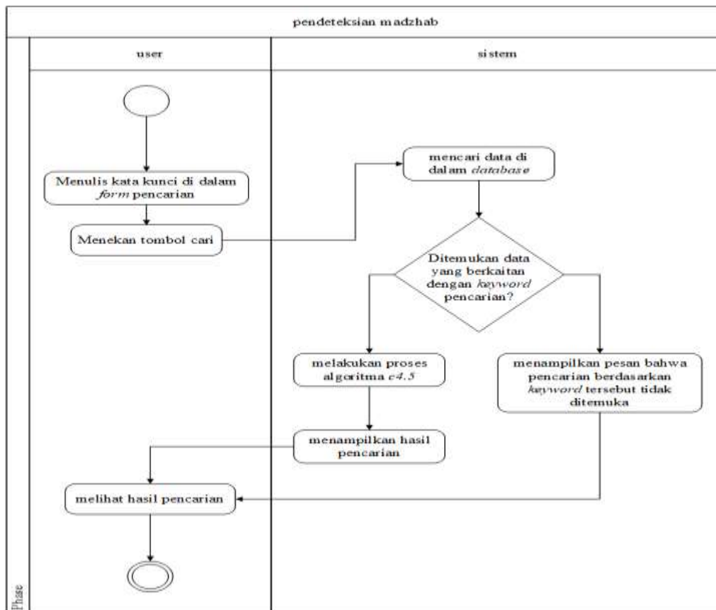
Gambar Activity Diagram Aplikasi Pendeteksiian Madzhab
